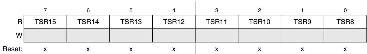
Figure 16-37. Time Stamp Register — High Byte (TSRH)
