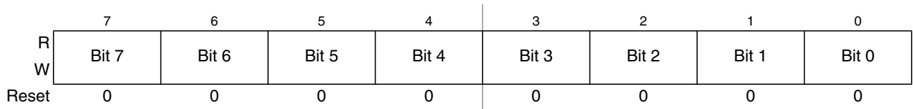
Figure 14-20. Timer Input Capture/Output Compare Register 0 Low (TC0)
