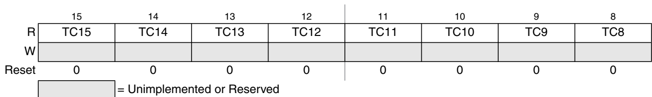
Figure 14-60. Timer Input Capture Holding Register 1 High (TC1H)
