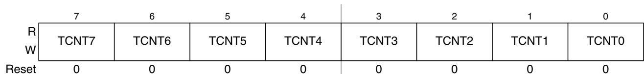
Figure 14-8. Timer Count Register Low (TCNT)
