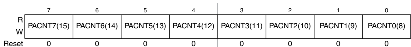
Figure 14-39. Pulse Accumulators Count Register 1 (PACN1)
