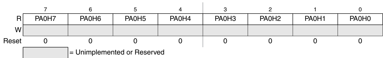
Figure 14-55. 8-Bit Pulse Accumulators Holding Register 0 (PA0H)
