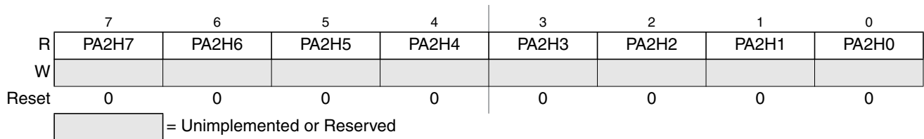
Figure 14-53. 8-Bit Pulse Accumulators Holding Register 2 (PA2H)
