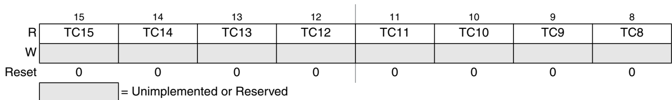
Figure 14-58. Timer Input Capture Holding Register 0 High (TC0H)
