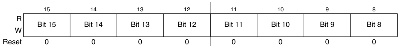
Figure 14-23. Timer Input Capture/Output Compare Register 2 High (TC2)
