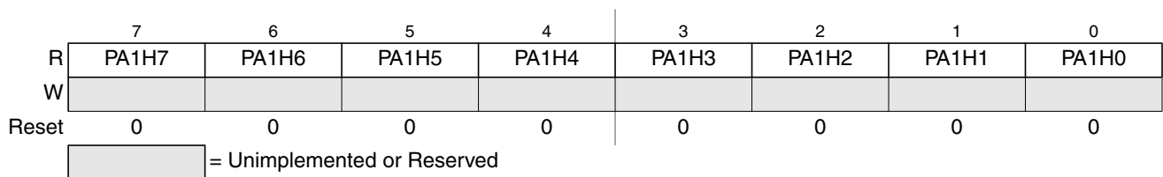
Figure 14-54. 8-Bit Pulse Accumulators Holding Register 1 (PA1H)
