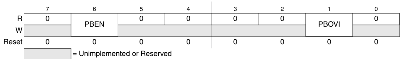
Figure 14-50. 16-Bit Pulse Accumulator B Control Register (PBCTL)
