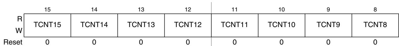
Figure 14-7. Timer Count Register High (TCNT)
