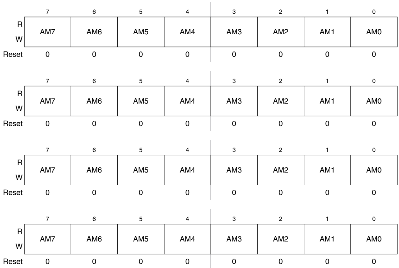
Figure 16-23. MSCAN Identifier Mask Registers (Second Bank) — CANIDMR4–CANIDMR7
