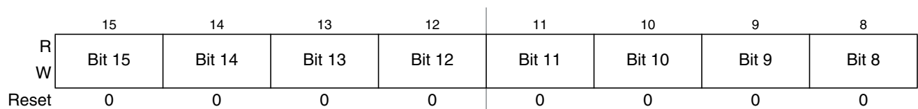
Figure 14-19. Timer Input Capture/Output Compare Register 0 High (TC0)
