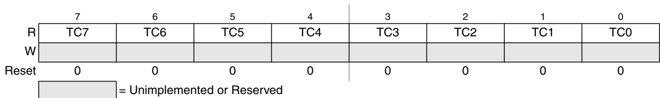
Figure 14-59. Timer Input Capture Holding Register 0 Low (TC0L)
