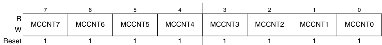
Figure 14-57. Modulus Down-Counter Count Register Low (MCCNT)
