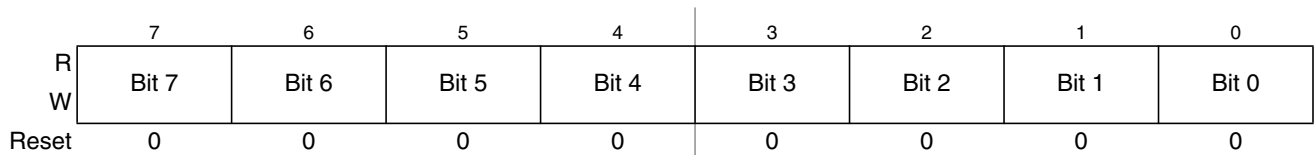
Figure 14-22. Timer Input Capture/Output Compare Register 1 Low (TC1)
