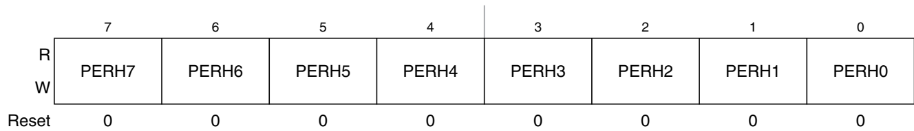
Figure 2-55. Port H Pull Device Enable Register (PERH)
