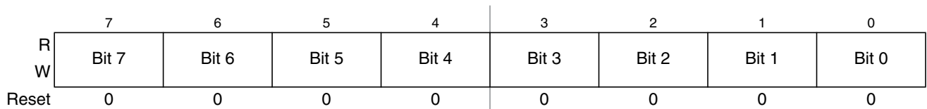
Figure 14-24. Timer Input Capture/Output Compare Register 2 Low (TC2)
