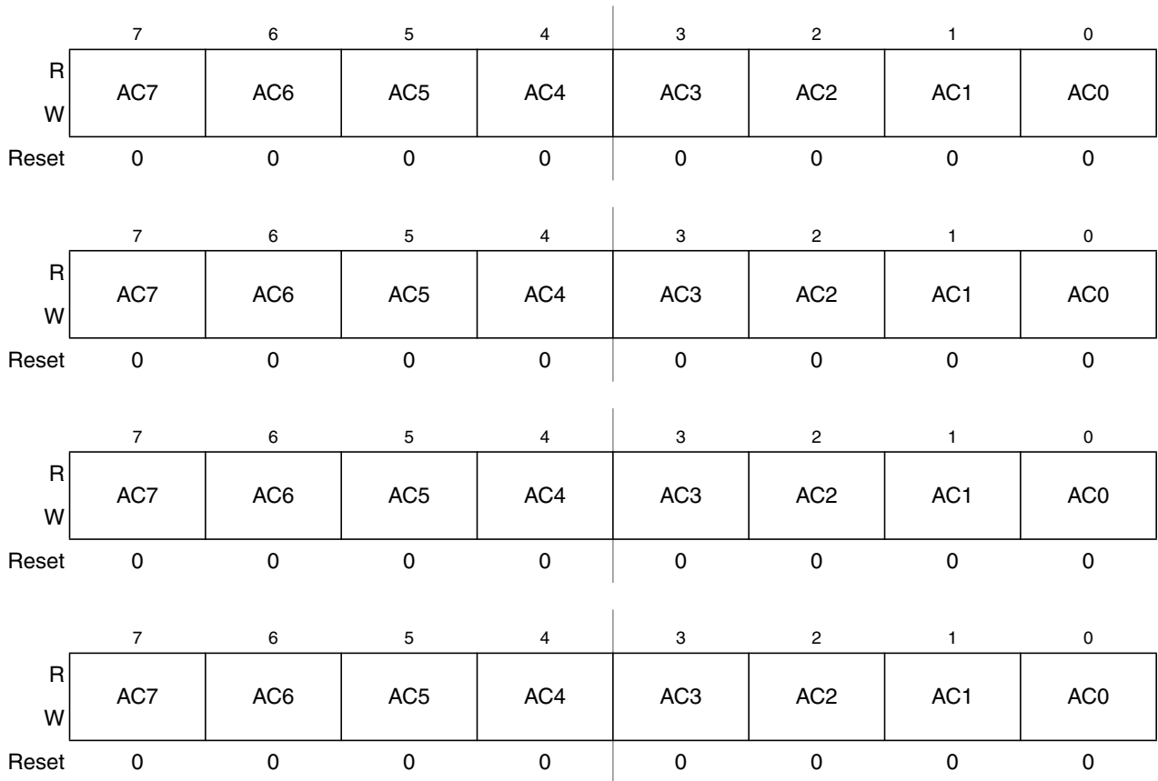
Figure 16-20. MSCAN Identifier Acceptance Registers (First Bank) — CANIDAR0–CANIDAR3
