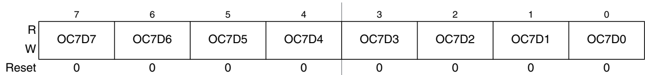
Figure 14-6. Output Compare 7 Data Register (OC7D)
