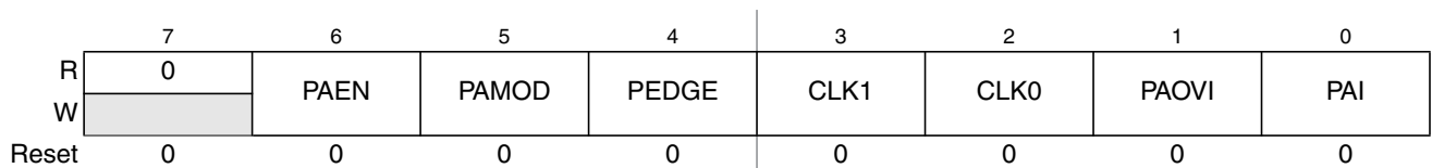
Figure 14-35. 16-Bit Pulse Accumulator Control Register (PACTL)
