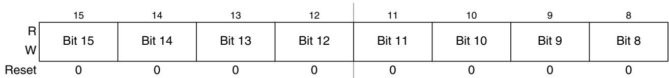
Figure 14-21. Timer Input Capture/Output Compare Register 1 High (TC1)
