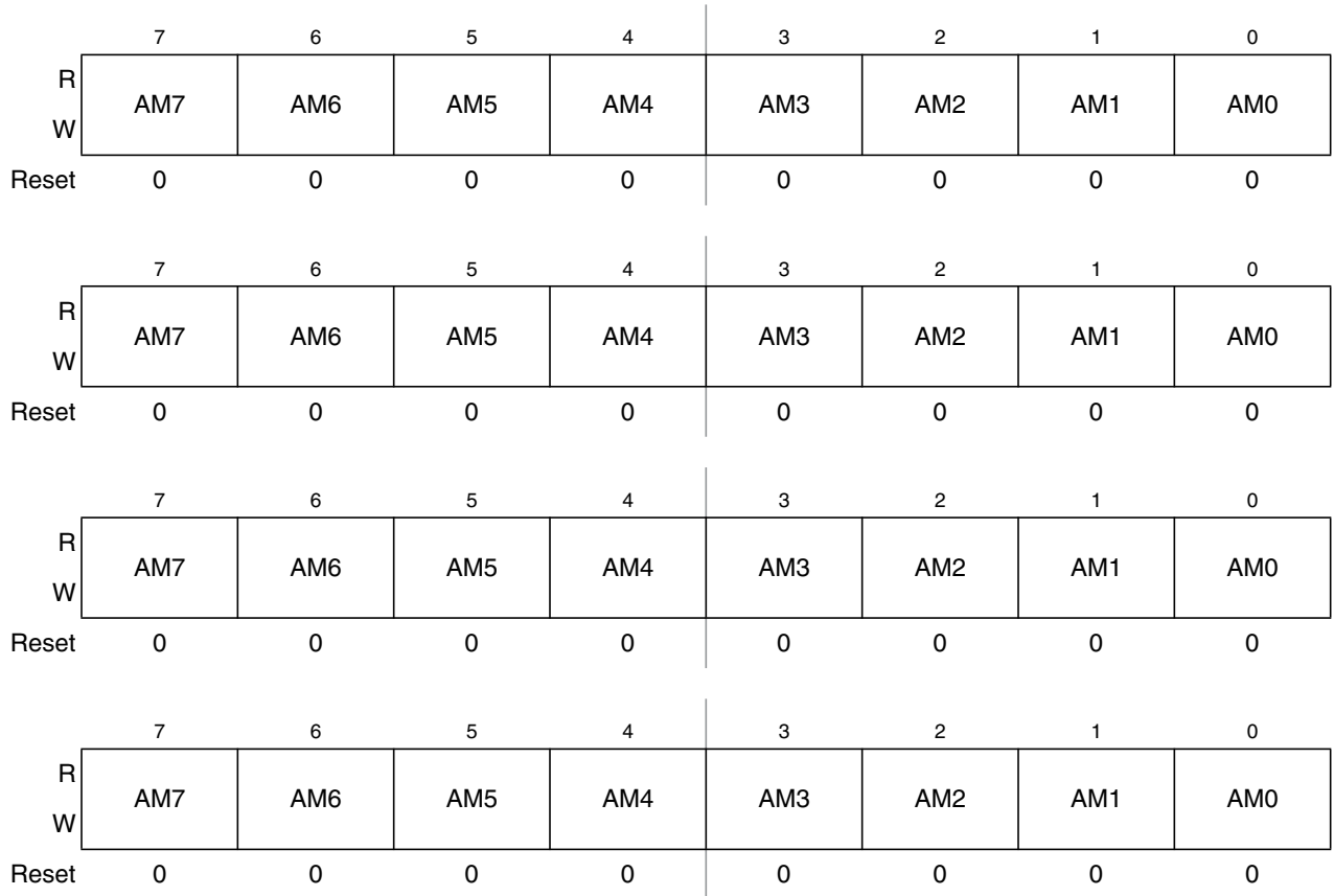
Figure 16-22. MSCAN Identifier Mask Registers (First Bank) — CANIDMR0–CANIDMR3
