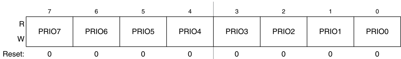
Figure 16-36. Transmit Buffer Priority Register (TBPR)
