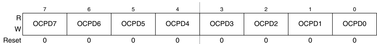
Figure 14-47. Output Compare Pin Disconnect Register (OCPD)
