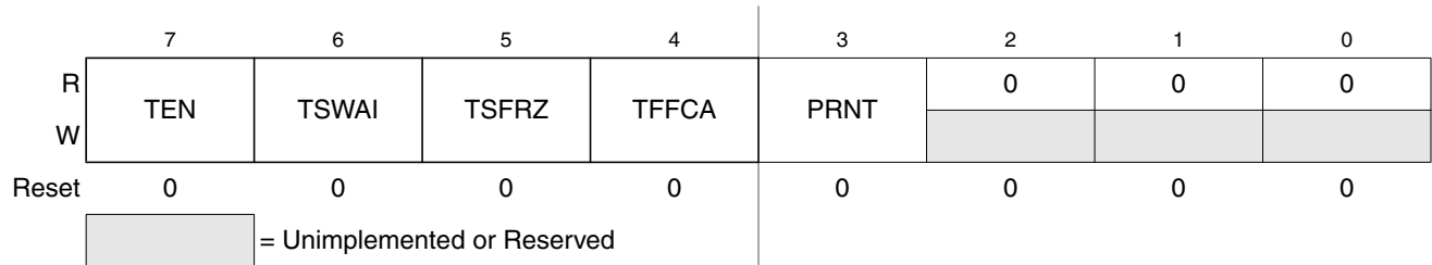
Figure 22-12. Timer System Control Register 1 (TSCR2)
