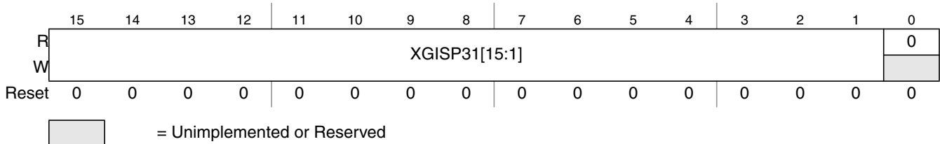
Figure 10-8. XGATE Initial Stack Pointer for Interrupt Priorities 3 to 1 (XGISP31)
